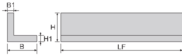
外徑墊高輔助刀座 Increased Outer Diameter Converter
