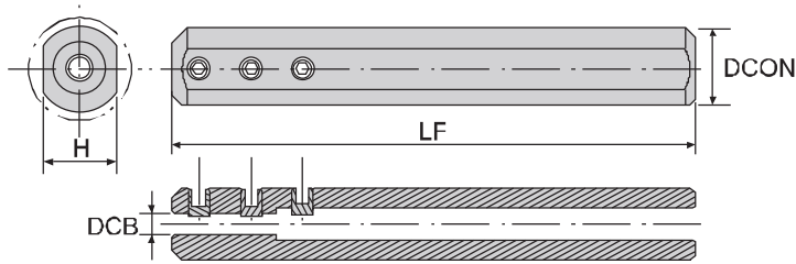
套筒 Sleeve 材質：鋼 Shank：Steel
