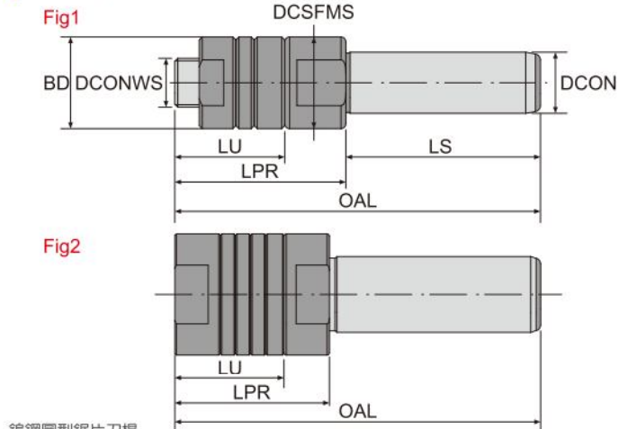
鎢鋼圓型鋸片刀桿 Carbide circular saw holder
